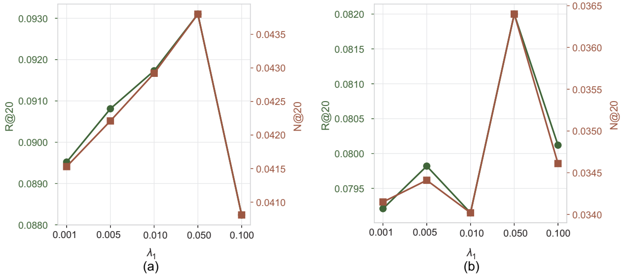
Fig. 4 Performance with different feature matching strengths \lambda_1 on the sports (a) and baby (b) datasets
